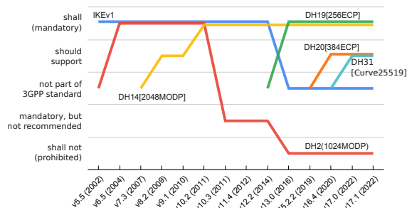
Figure 3: Development of the IPsec IKE Profile as defined in IETF TS 133.210 (IKE_SA_INIT) [23] Note: LTE started with v8, and IKEv1 has been phased out since v12.
